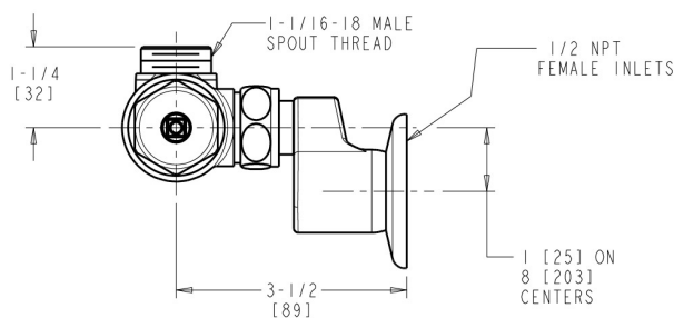
SIDE VIEW
