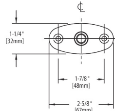
FLANGE DETAIL
